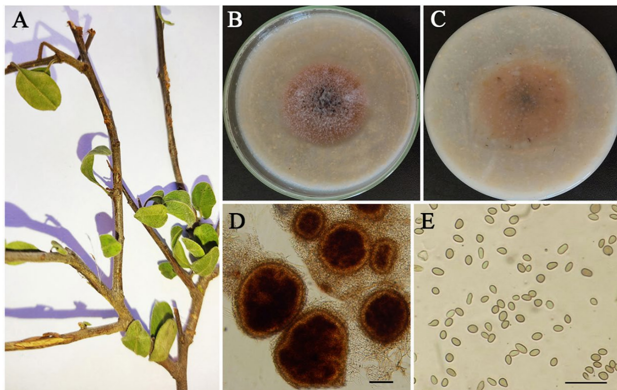
Fig. 8. Paramicrosphaeropsis salandica (SCUA-Is-D8). (A) Stem canker on Rhamnus persica , (B, C) Colony on OA after 9 d at 25 °C (top and reverse), (D) Pycnidia, (E) Conidia. Scale bars: (D) 70 \mu\text{m} , (E) 20 \mu\text{m} .
