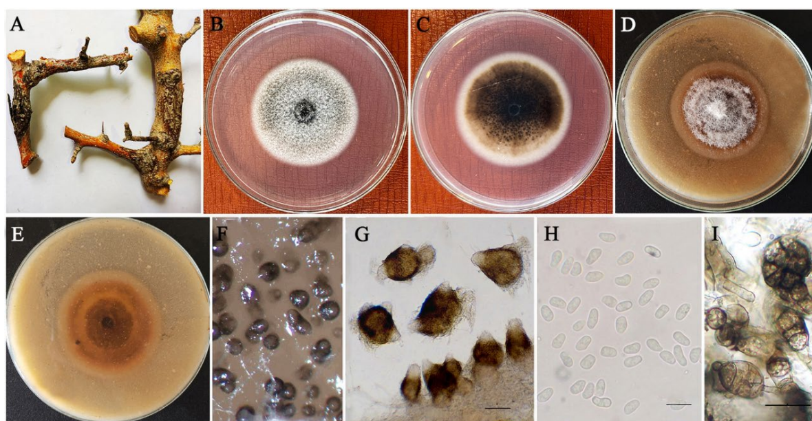
Fig. 3. Didymella microchlamydospora (SCUA-Is-A12). (A) Stem canker on Crataegus sp., Colonies on PDA (B, C), and OA (D, E) after 7 d at 25 °C (top and reverse), (F, G) Pycnidia, (H) Conidia, (I) Chlamydospores. Scale bars: (G) 70 µm, (H) 7 µm, (I) 20 µm.
