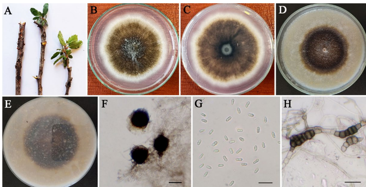
Fig. 4. Didymella pinodella (SCUA-Is-E7). (A) Stem canker on Cerasus microcarpa , Colonies on PDA (B, C), and OA (D, E) after 7 d at 25 °C (top and reverse), (F) Pycnidia, (G) Conidia, (H) Chlamydospores. Scale bars: (F) 70 \mu\text{m} , (G) 20 \mu\text{m} , (H) 20 \mu\text{m} .
