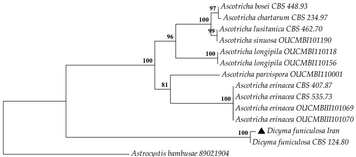
Fig. 3. Phylogenetic tree generated from a Maximum likelihood inference based on combined ITS and \beta -tubulin datasets. Maximum likelihood bootstrap are indicated at the nodes. Black triangle refer to Iranian isolate.
